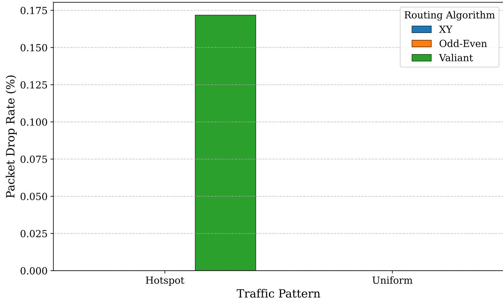
Packet Loss Comparison (4x4 Torus)
