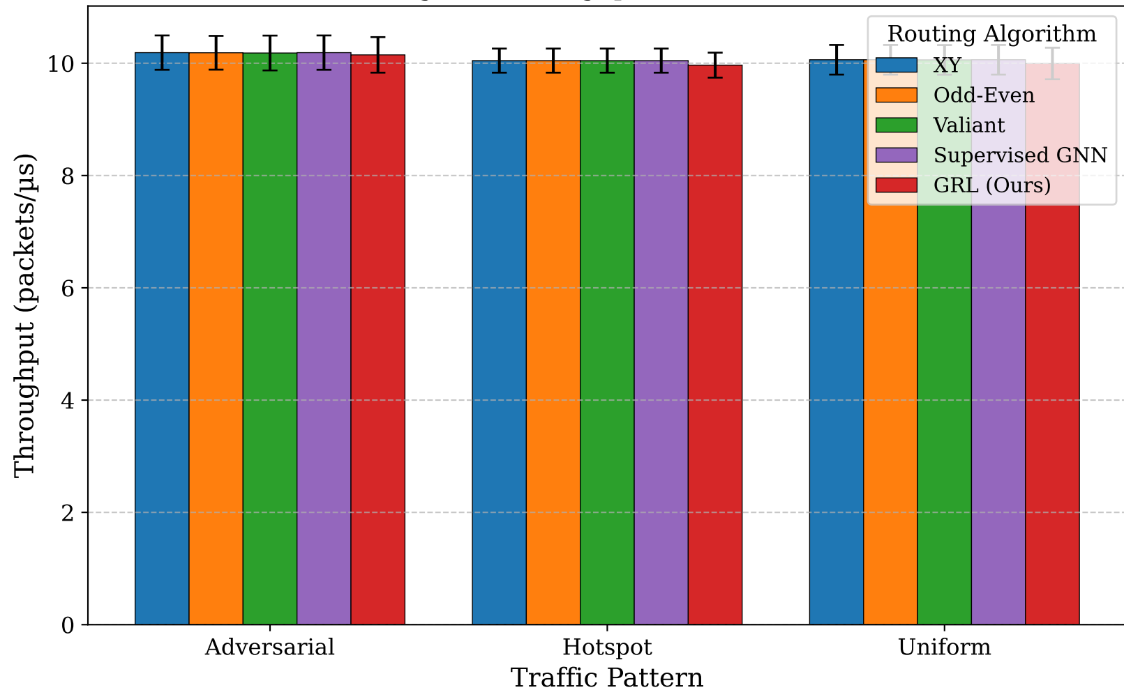
Fig. 10: Throughput (8×8 Torus)
