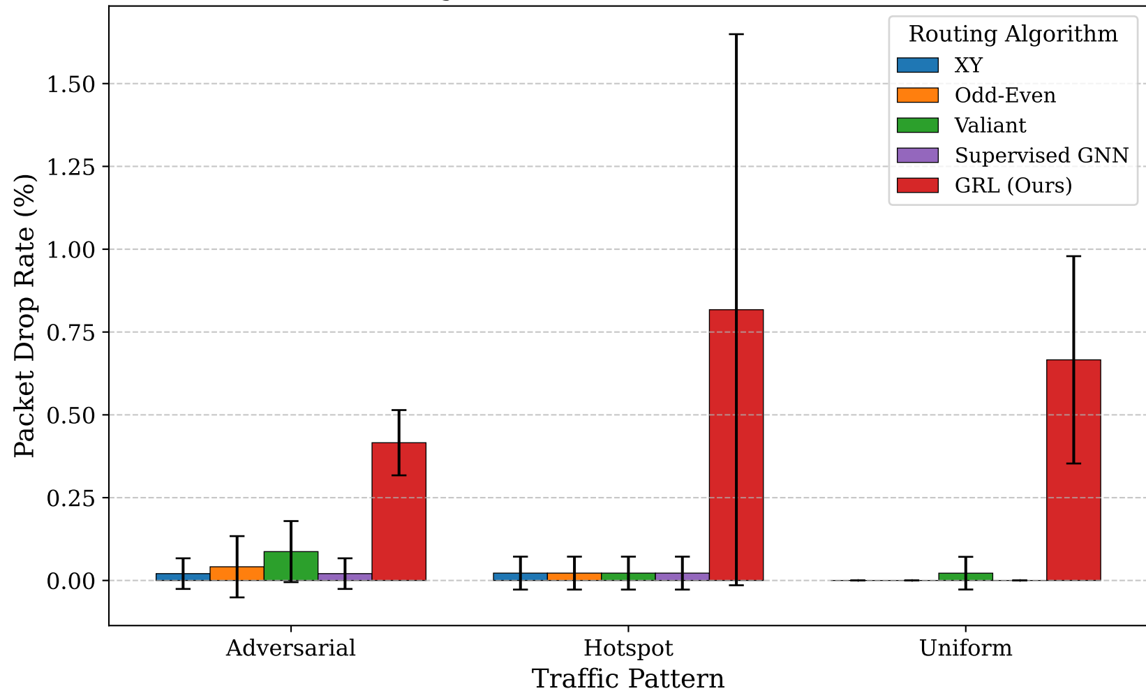
Fig. 11: Packet Loss (8×8 Torus)
