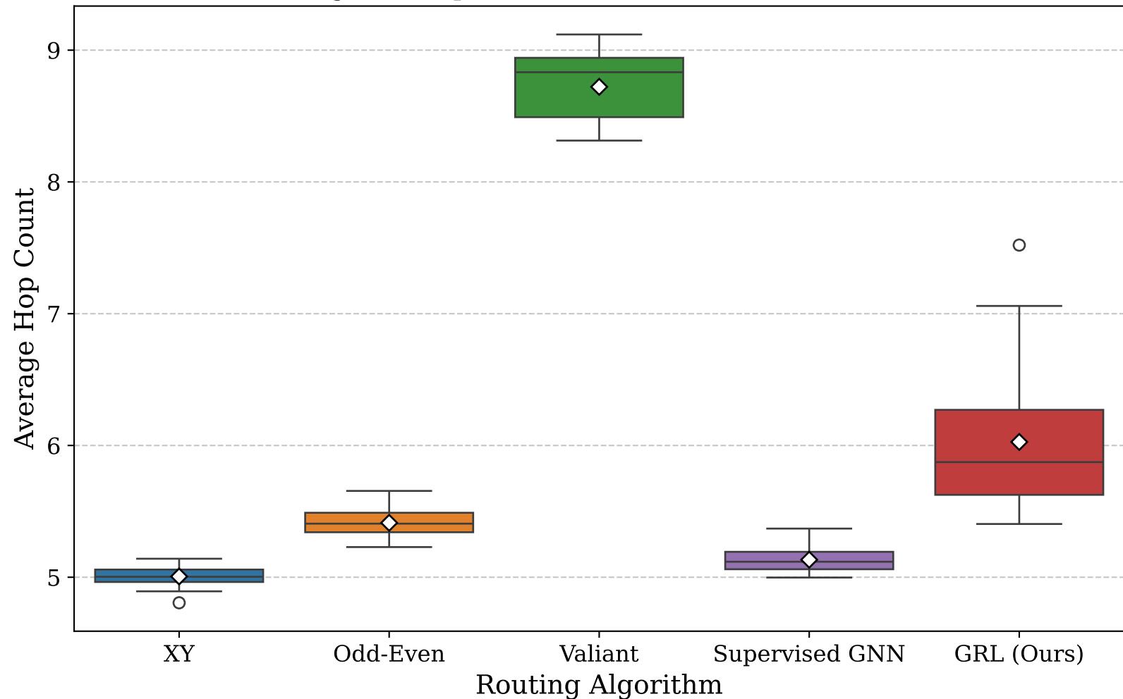
Fig. 12: Hop Count Distribution (8×8 Torus)
