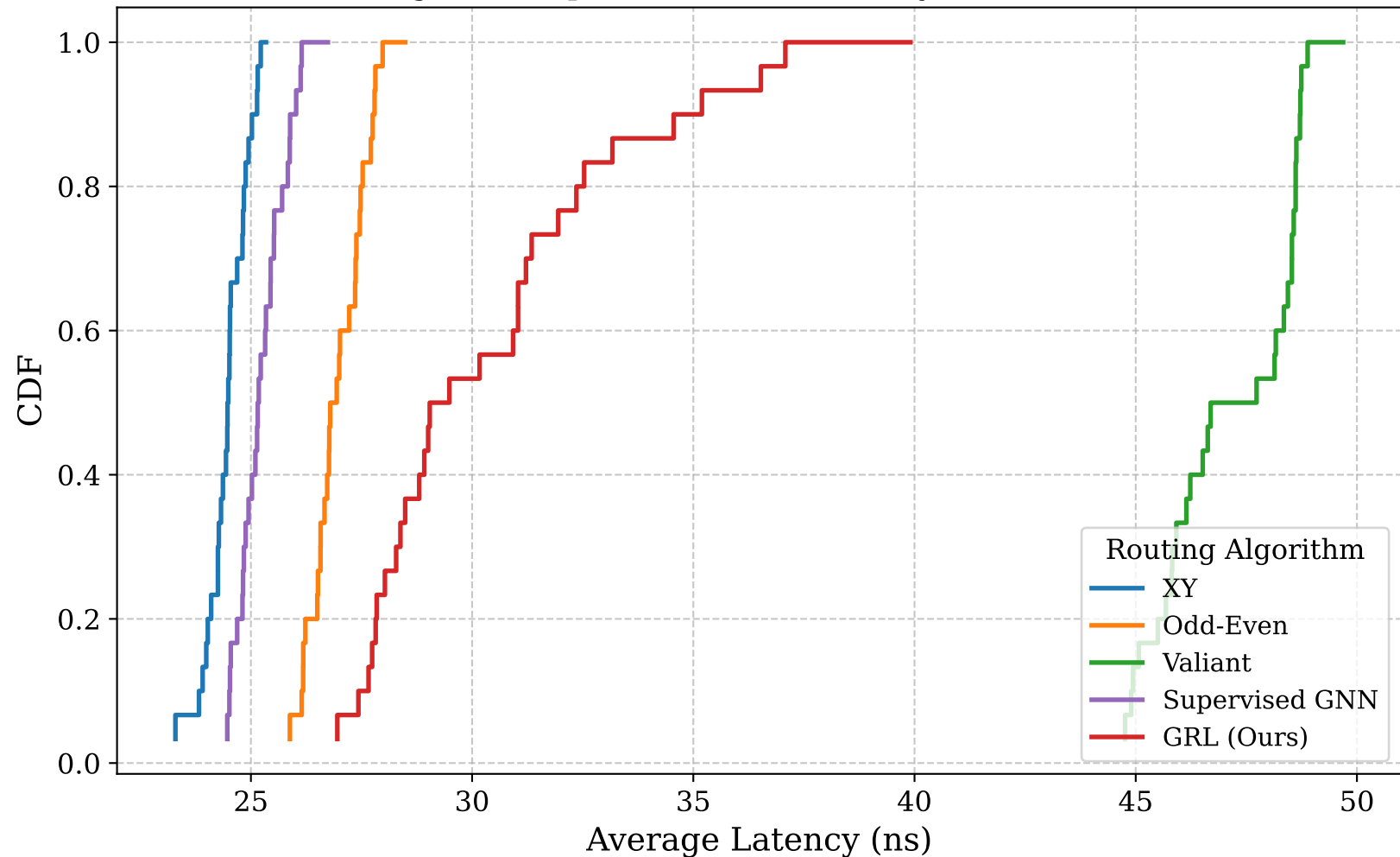
Fig. 13: Empirical CDF of Latency (8×8 Torus)
