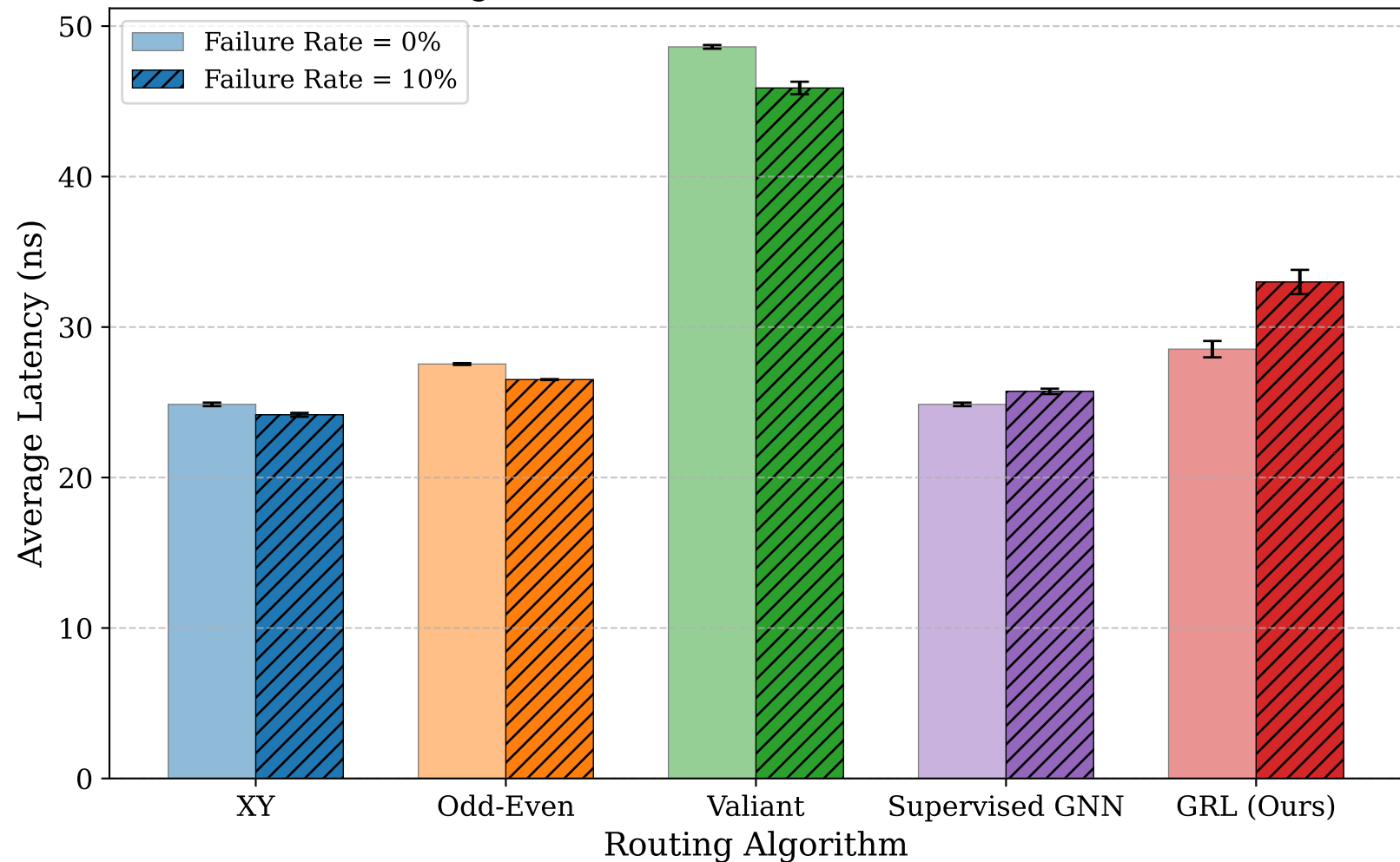
Fig. 14: Failure Resilience (8×8 Torus)
