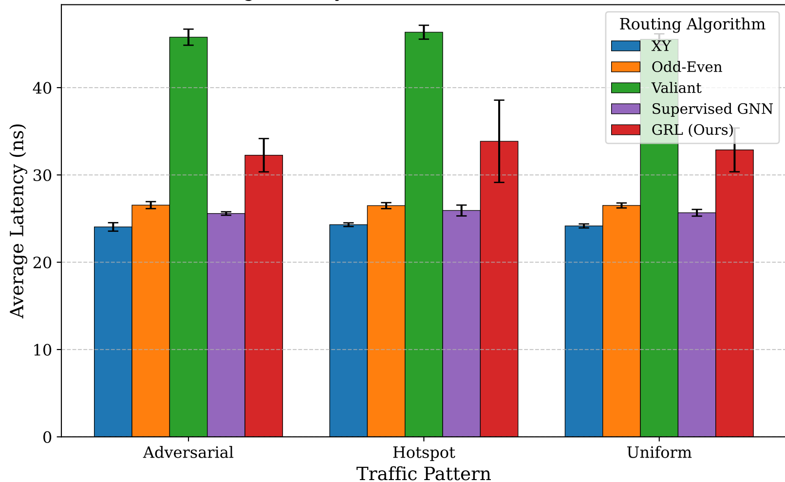
Average Latency — 10% Link Failures (8×8 Torus)
