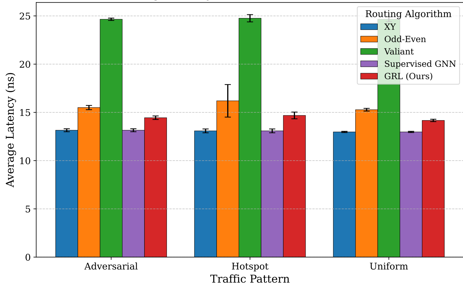
Average Latency — Normal Traffic (4×4 Torus)
