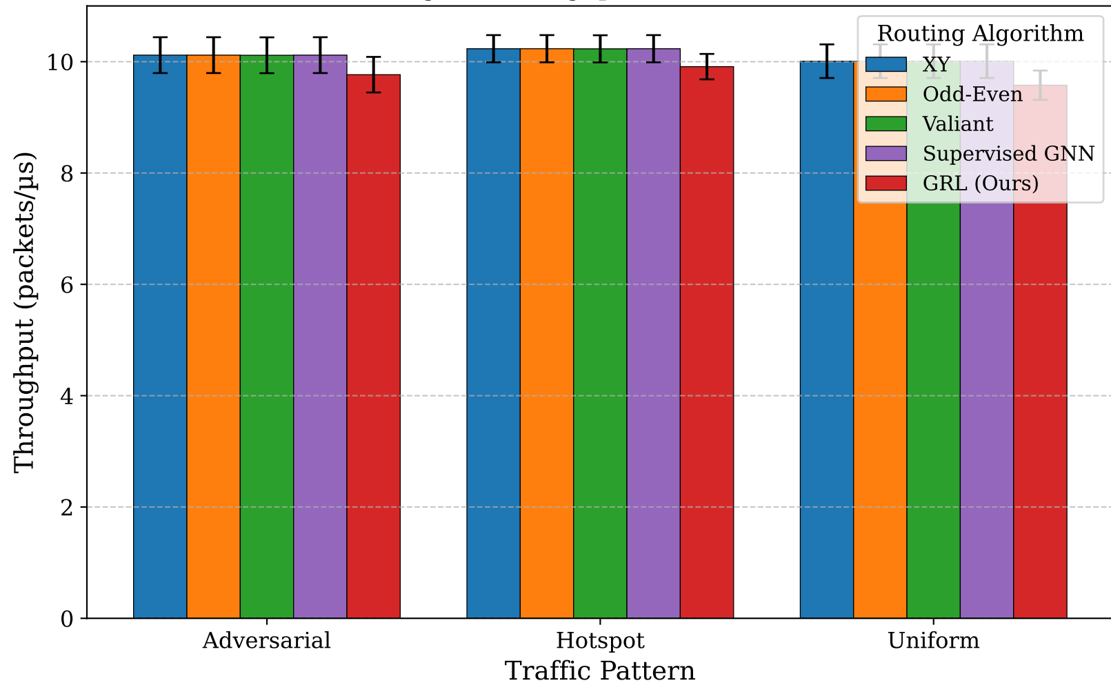
Fig. 2: Throughput (4×4 Torus)
