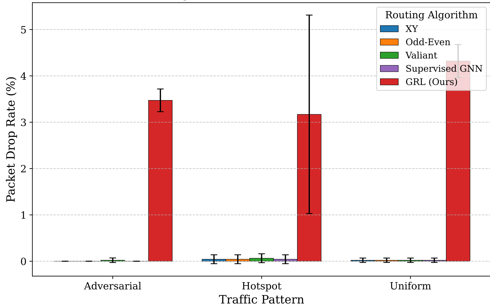
Fig. 3: Packet Loss (4×4 Torus)
