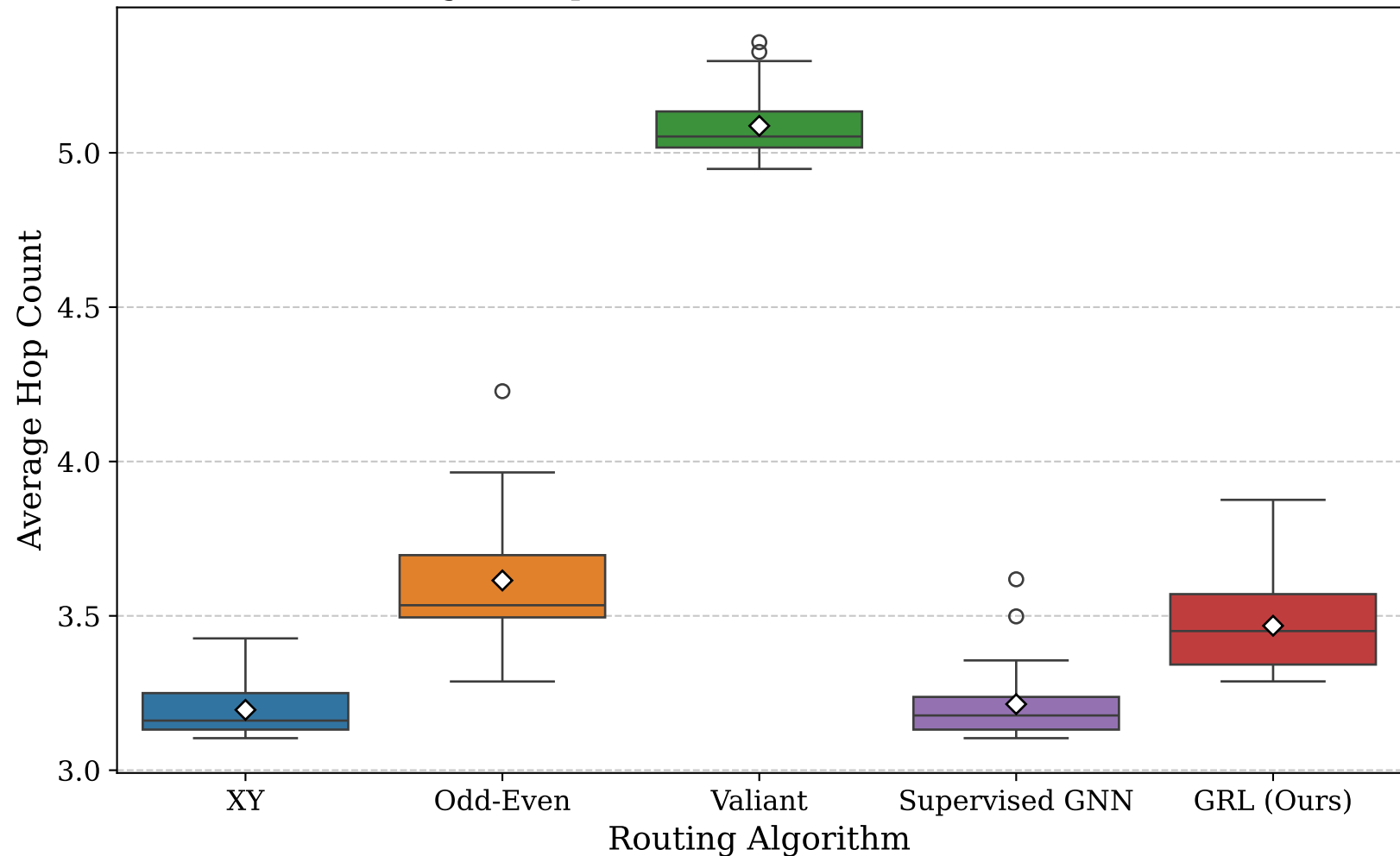
Fig. 4: Hop Count Distribution (4×4 Torus)
