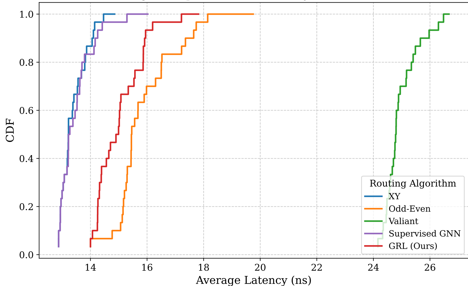
Fig. 5: Empirical CDF of Latency (4×4 Torus)
