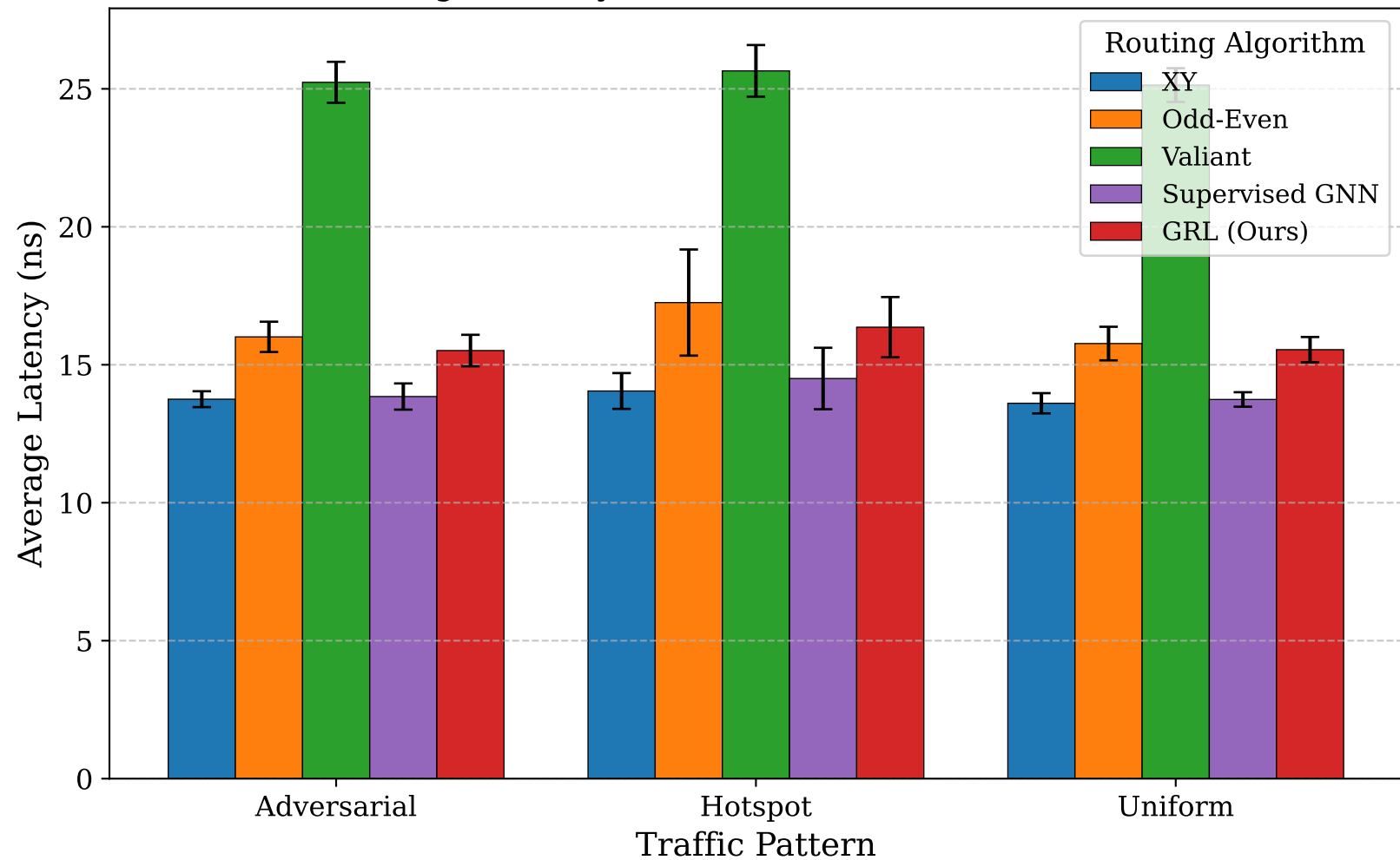
Average Latency — 10% Link Failures (4×4 Torus)
