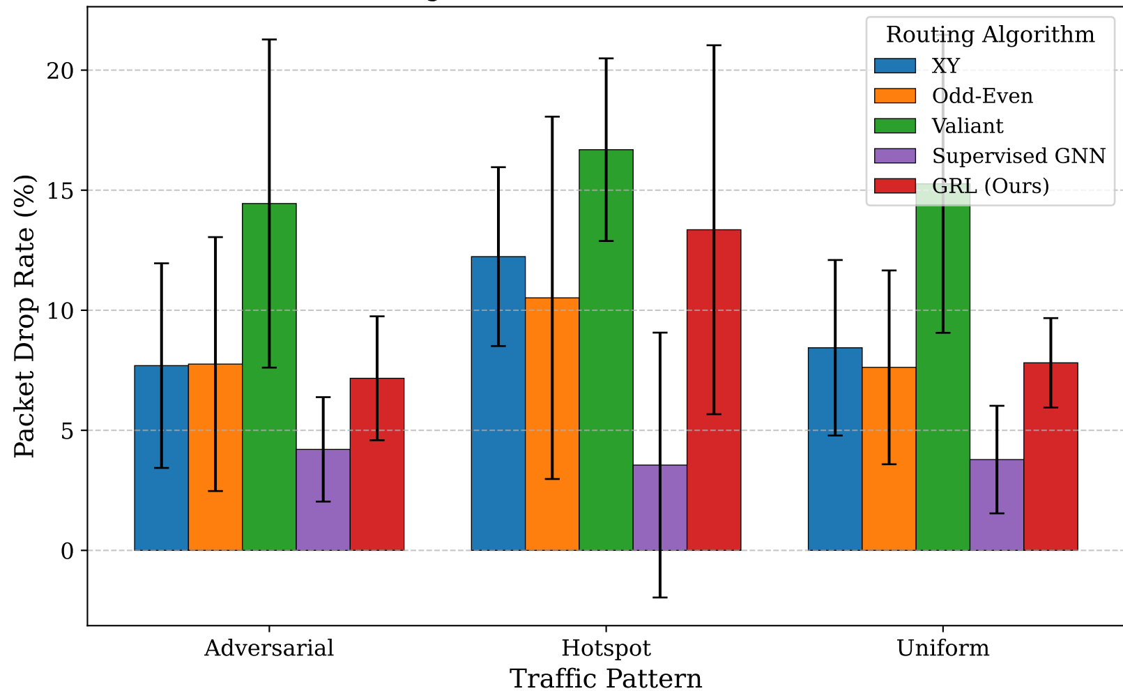
Fig. 8: Packet Loss (4x4 Torus)
