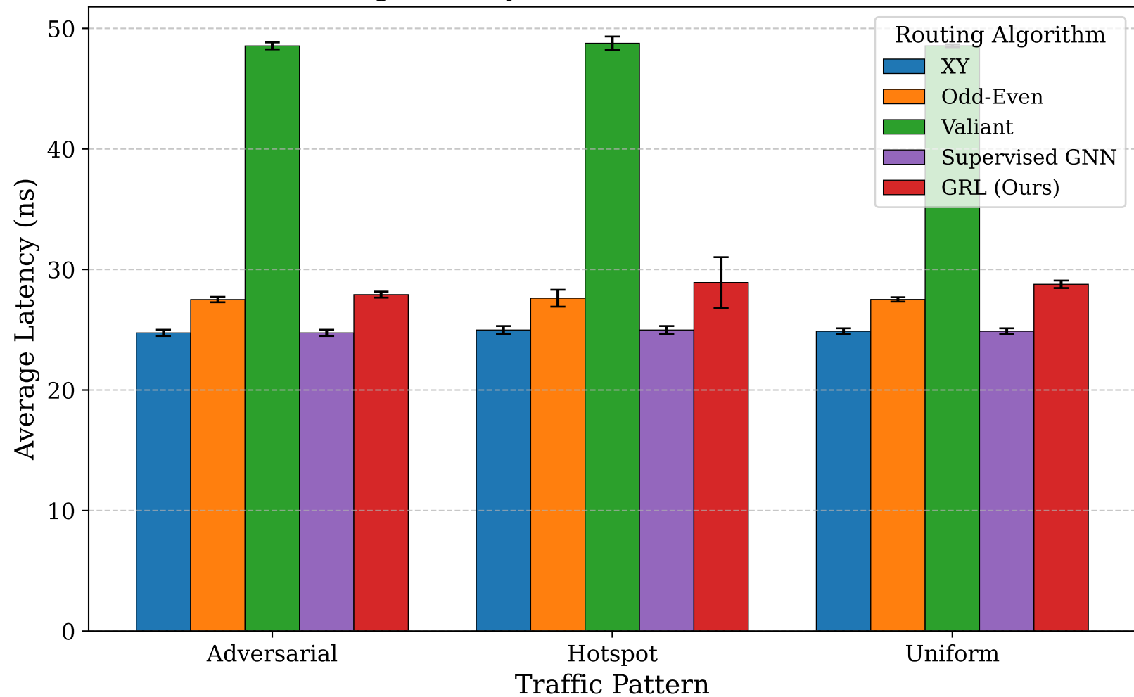
Average Latency — Normal Traffic (8×8 Torus)
