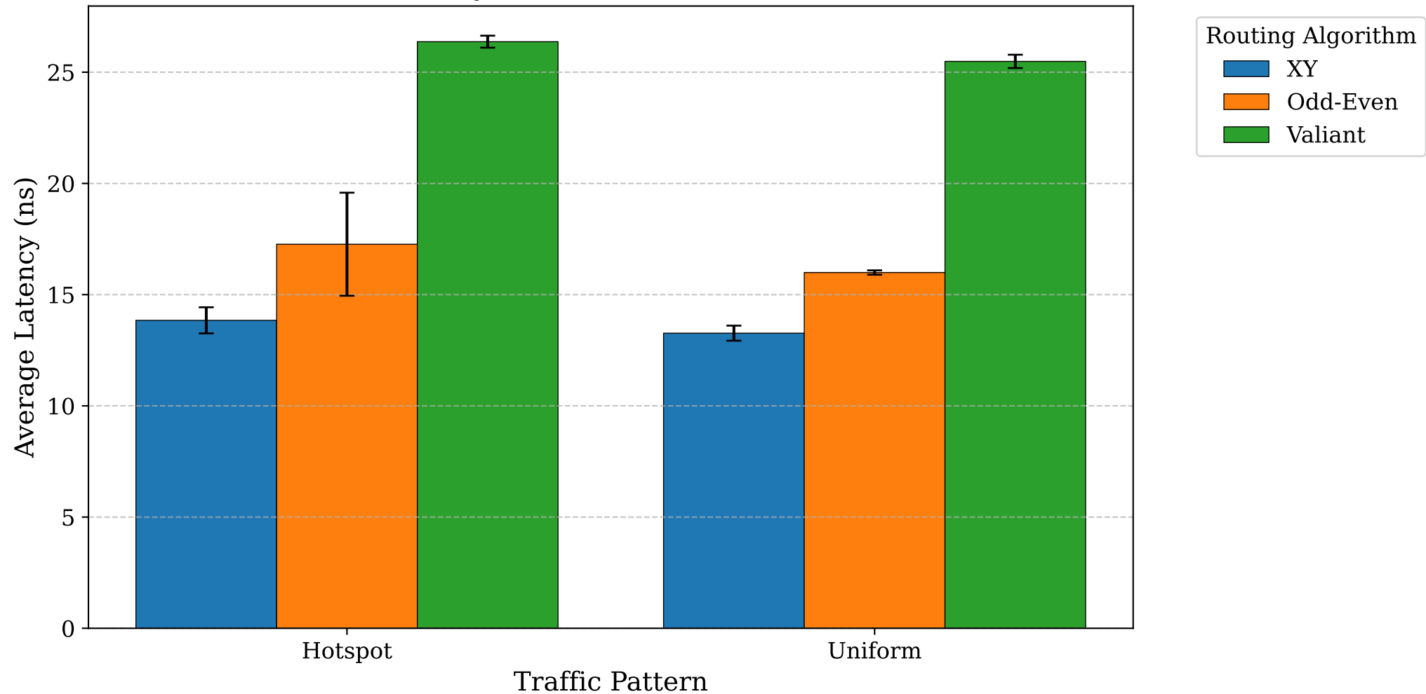
Latency: Link Failures (4x4 Torus)
