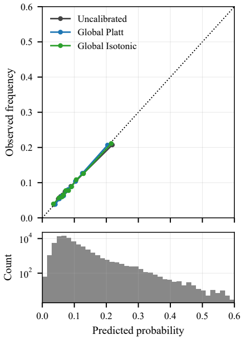
LR
