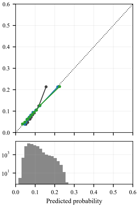
RF
