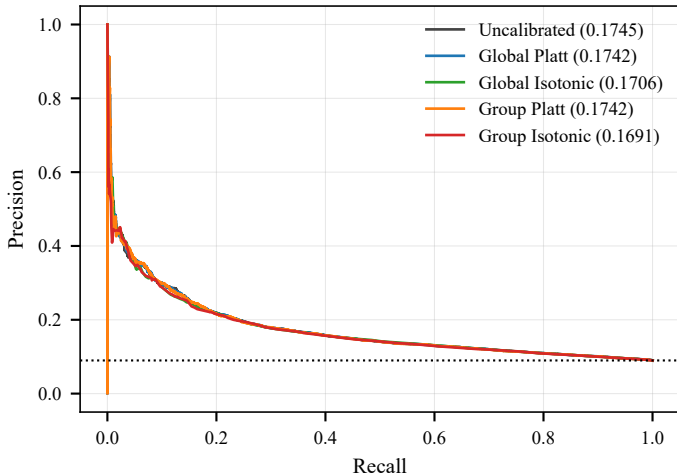
Precision-Recall — HGB
