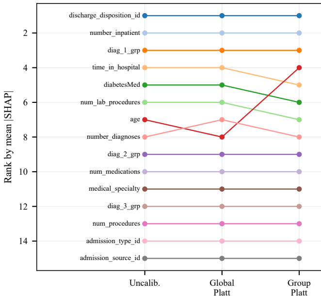
Attribution stability ( \tau=0.993 )
