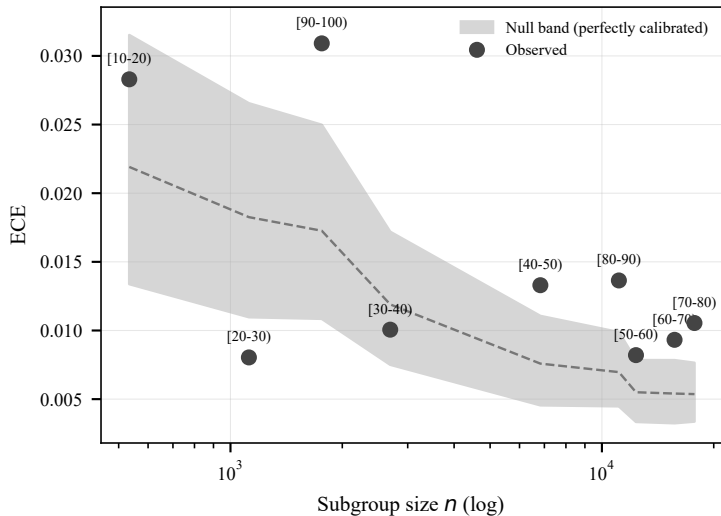
HGB — Uncalibrated
