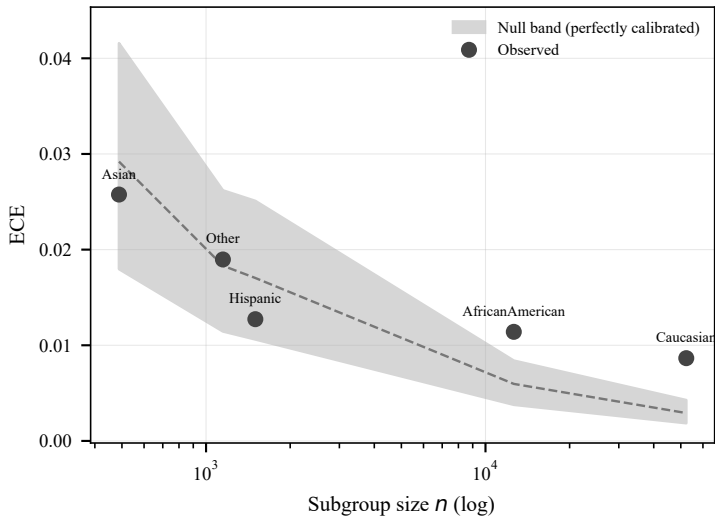
HGB — Uncalibrated
