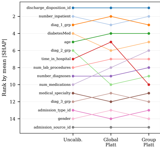
Attribution stability ( \tau=0.963 )
