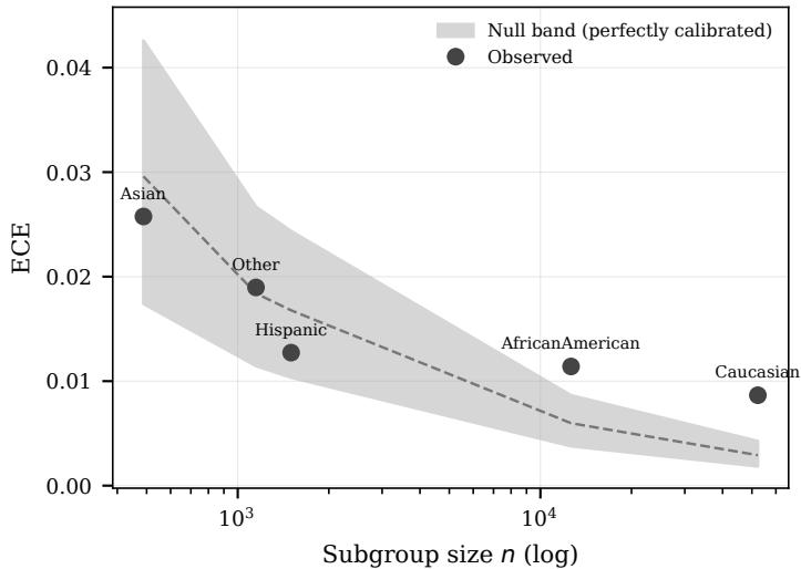
HGB — Uncalibrated
