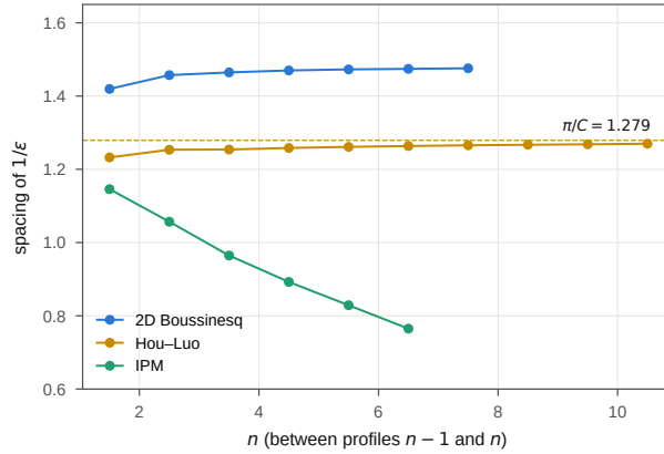
Supplementary Fig. 3. Spacings of consecutive profiles in 1/\varepsilon . A stalled layer of fixed extent gives increasing spacings (2D Boussinesq, Hou-Luo; dashed: the Hou-Luo asymptote \pi/C = 1.279 obtained from the \lambda \rightarrow 1 limit problem); the receding layer of IPM gives contracting spacings.
