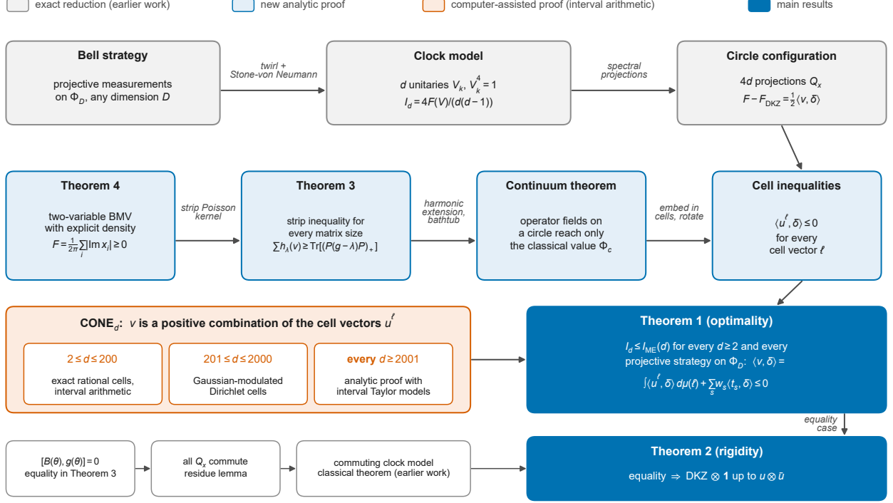
Figure 1: Architecture of the proof of Theorems 1 and 2: the exact reduction (Section 3.3), the analytic chain (Sections 3.4–3.6; the density of Theorem 4 is denoted F in the figure and \rho in the text), the certified cone condition (Section 3.7) and the equality case (Section 3.8).
