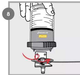
Install MEMOLUB PLCD on PLCD Memo.
