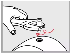
Screw BSP 1/8 fitting on lube point.
