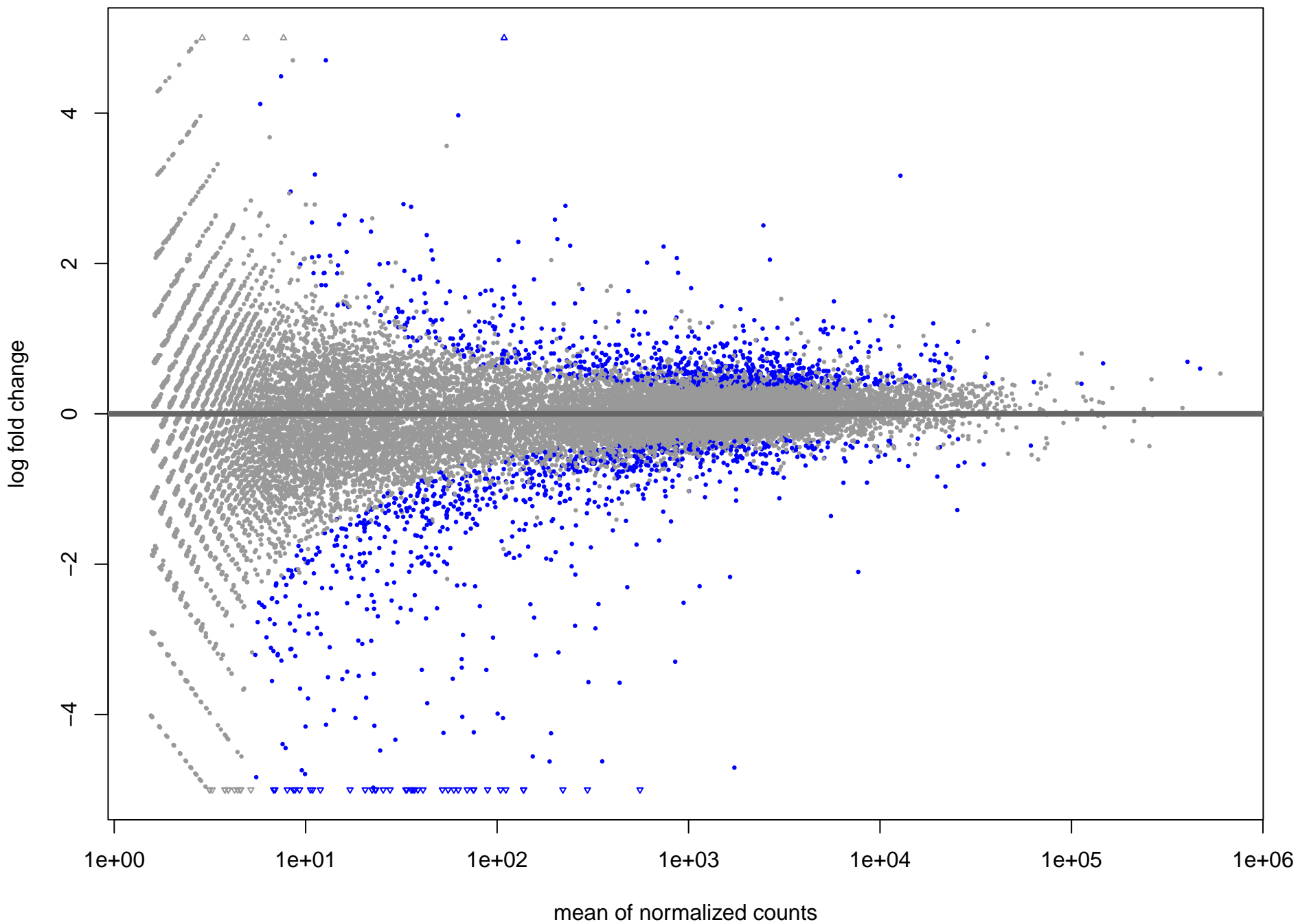
MA Plot: BT549/BT540 KO vs Control
