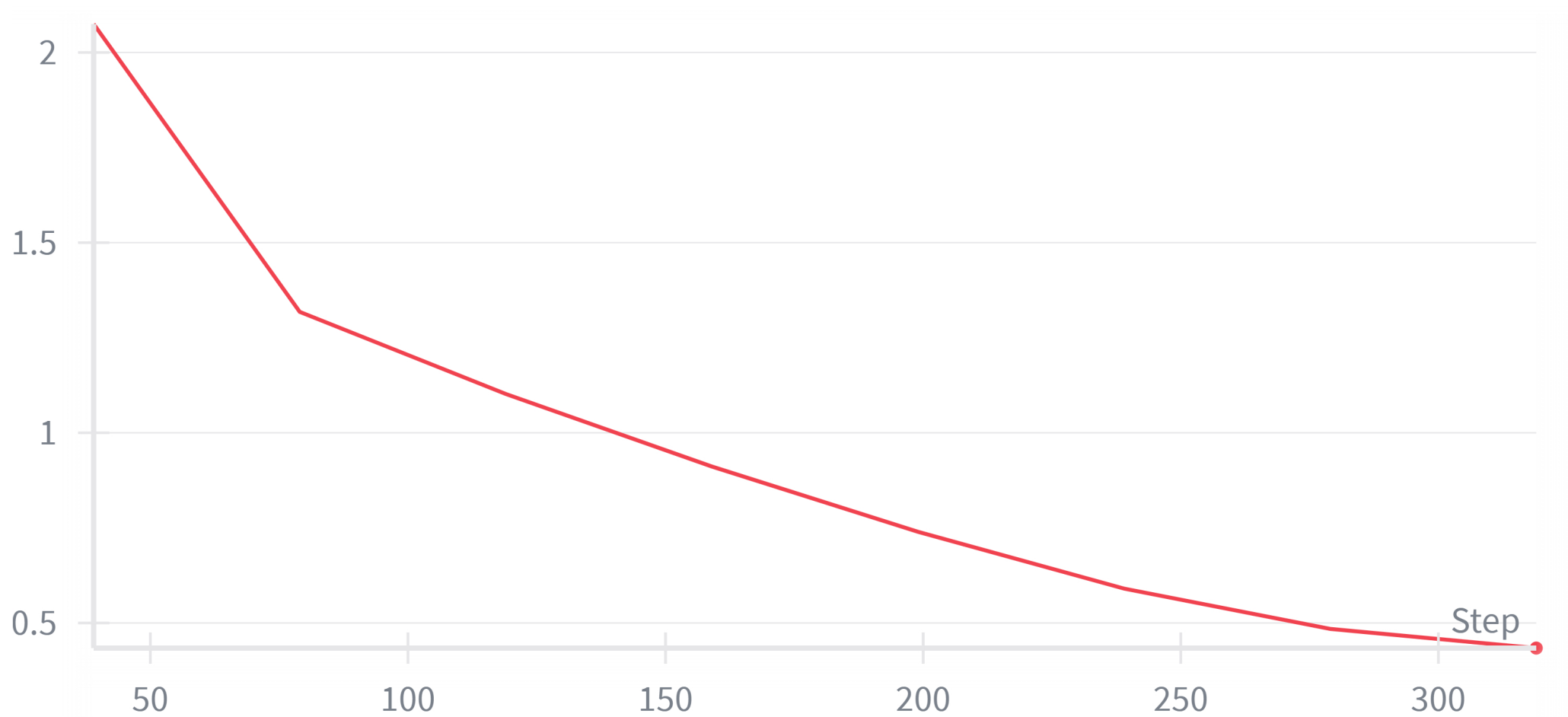
train/epoch_loss
