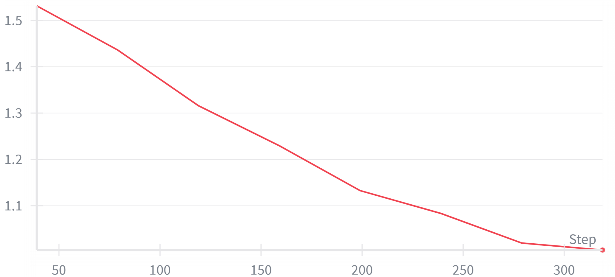
val/loss
