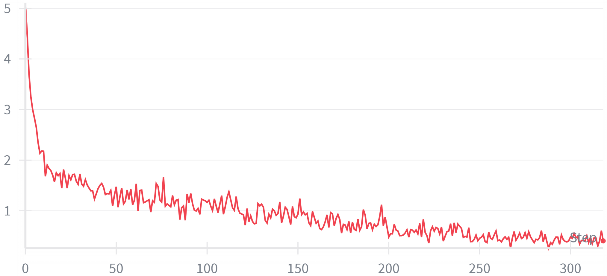
train/loss
