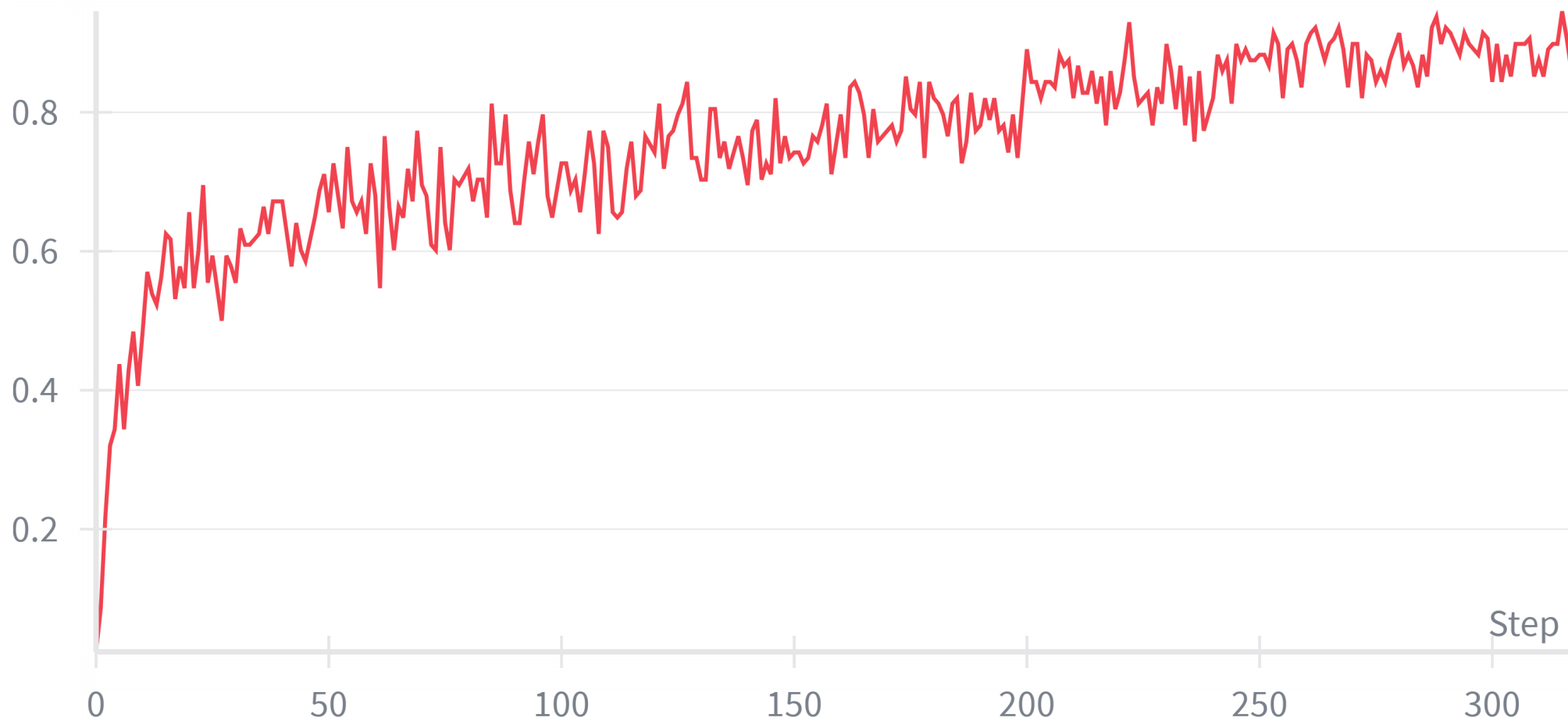
train/acc
