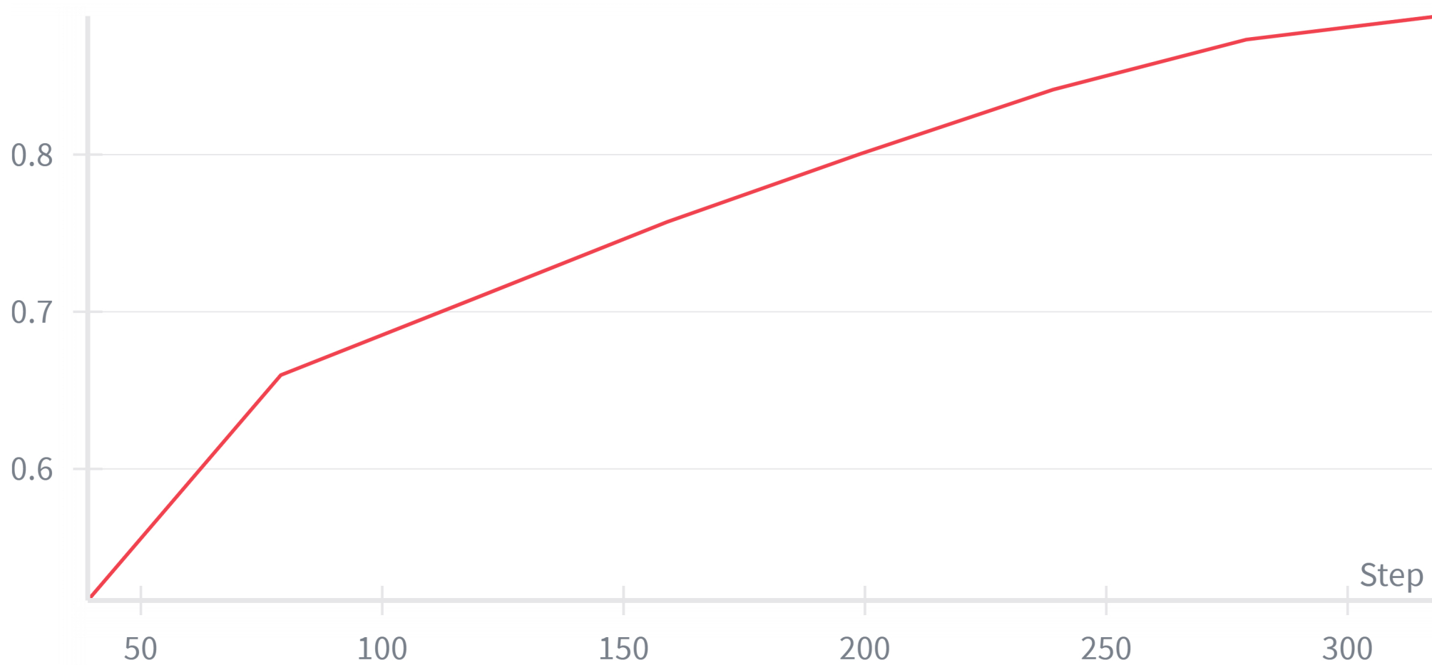
train/epoch_acc
