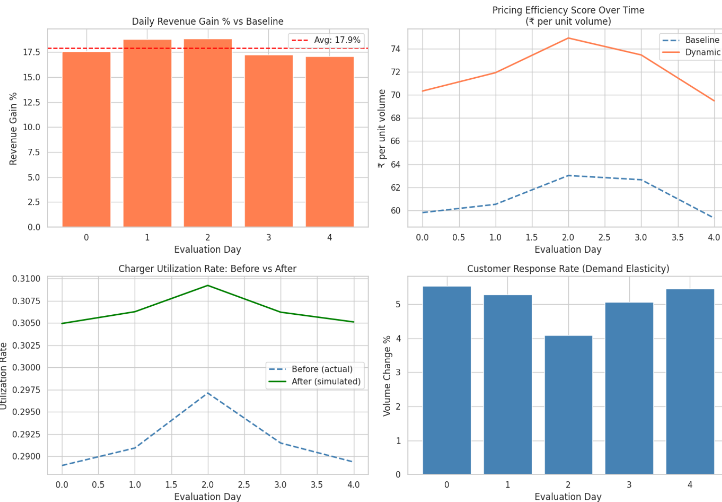
Monitoring & Learning Agent : Feedback Loop Performance
