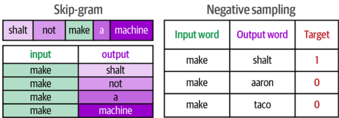
Figure 2-14. Skip-gram and negative sampling are two of the main ideas behind the word2vec algorithm and are useful in many other problems that can be formulated as token sequence problems.
