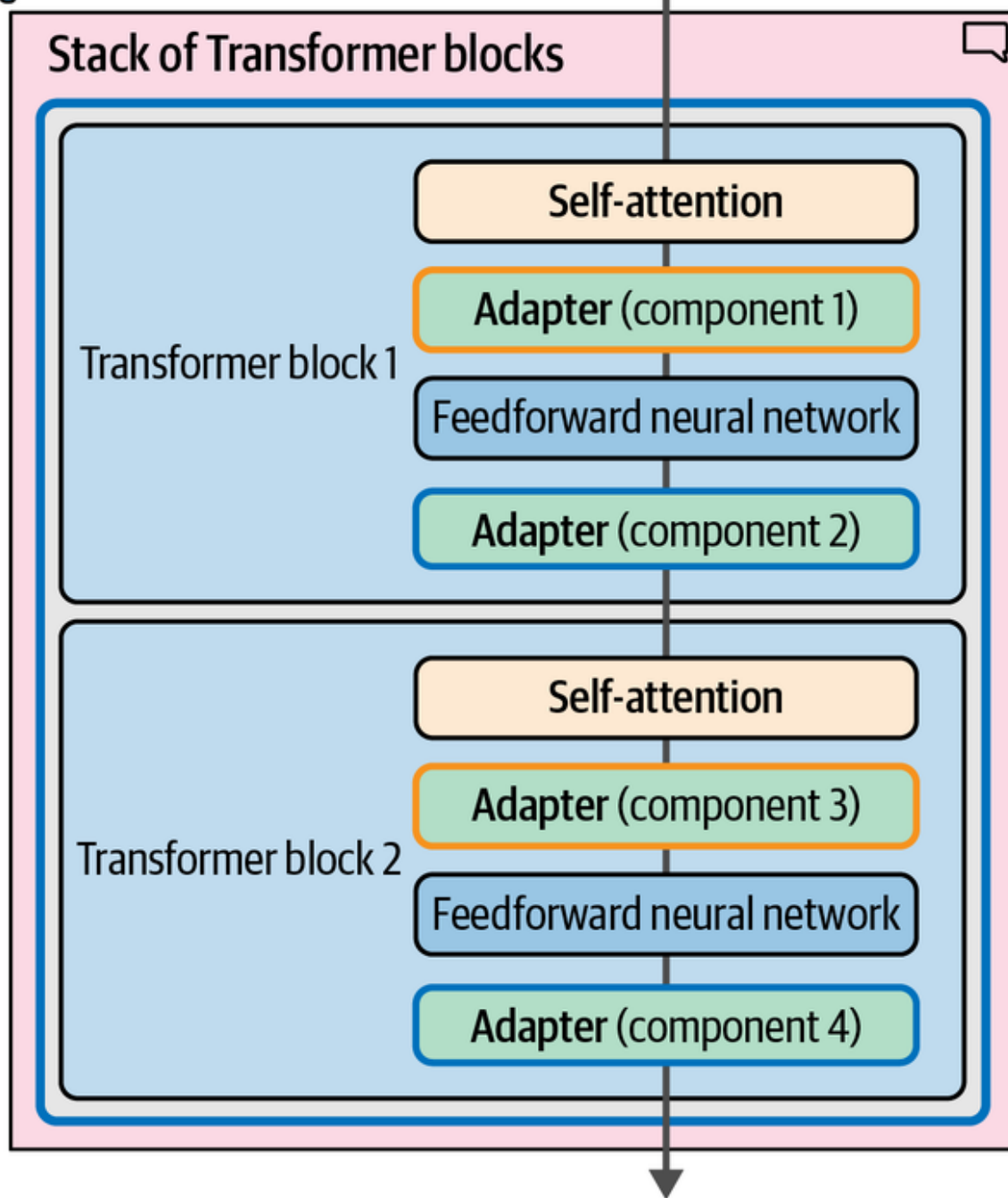
Figure 12-9. Adapter components span the various Transformer blocks in the model.
