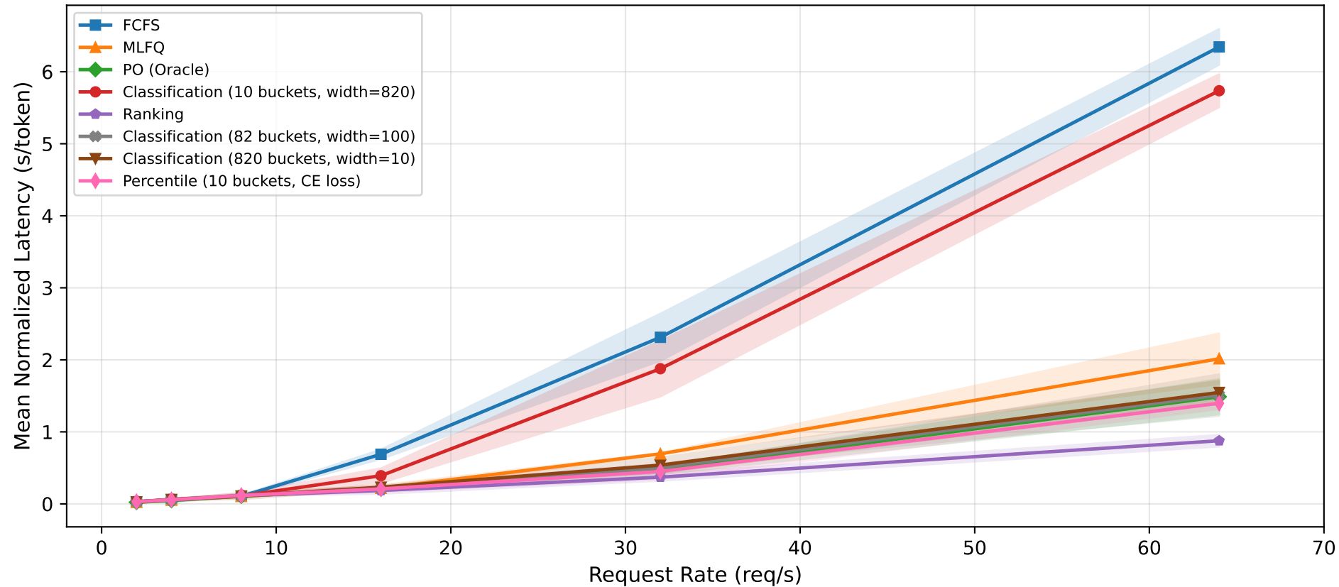
Scheduler Comparison with 95% CI — LMSYS-Chat-1M LLaMA-3-8B, 1 A100 80GB GPU (n=3 runs)
