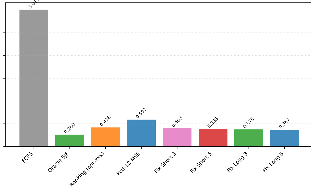
ShareGPT — rate=64
