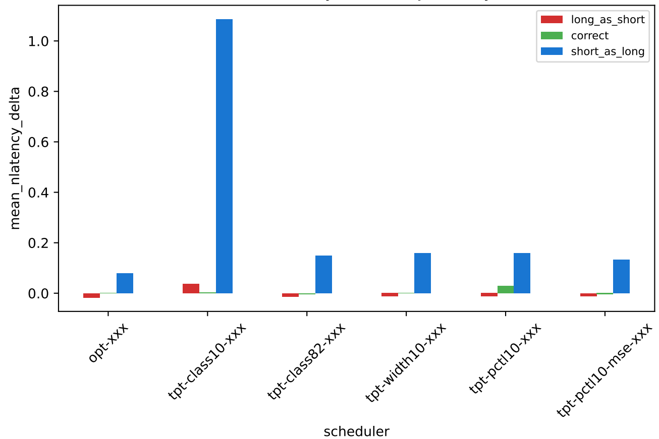
Mean nLatency delta vs SJF -- lmsys
