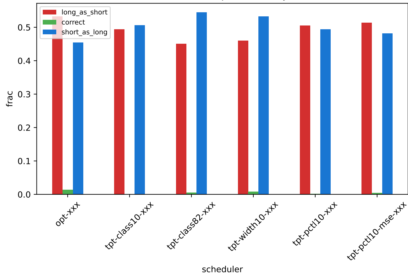
Fraction of requests -- lmsys
