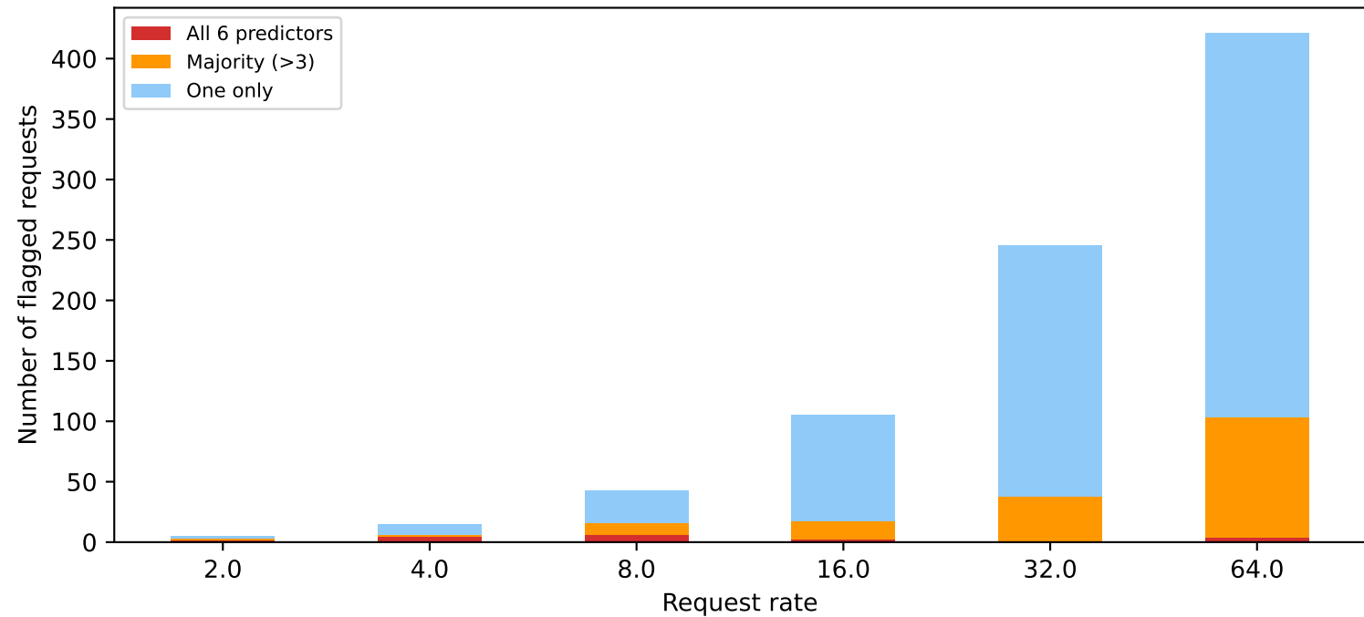
Outlier overlap (top 5% damage) -- lmsys
