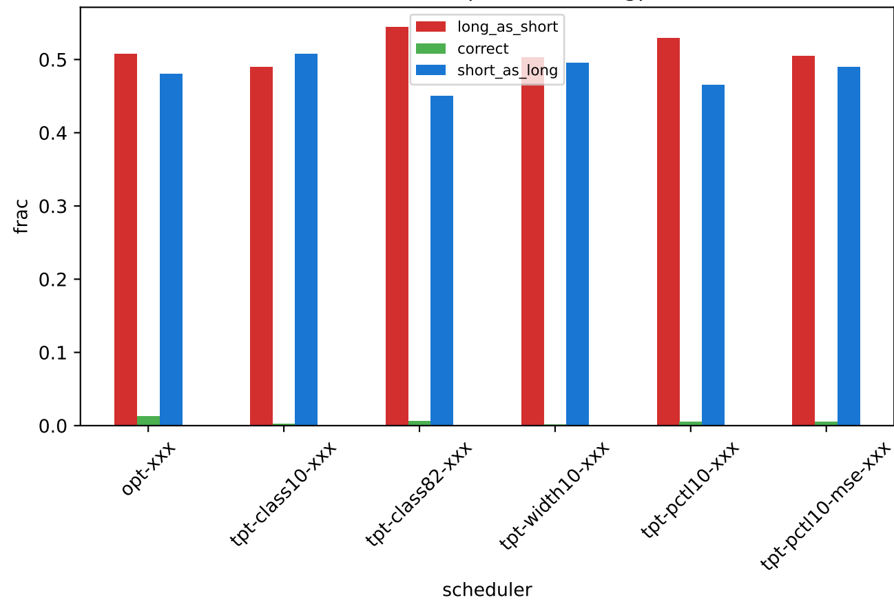
Fraction of requests -- sharegpt
