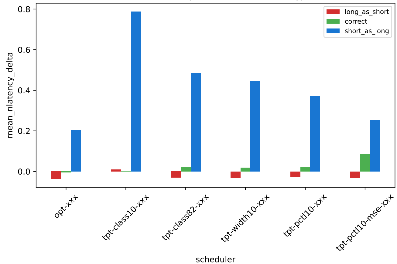
Mean nLatency delta vs SJF -- sharegpt
