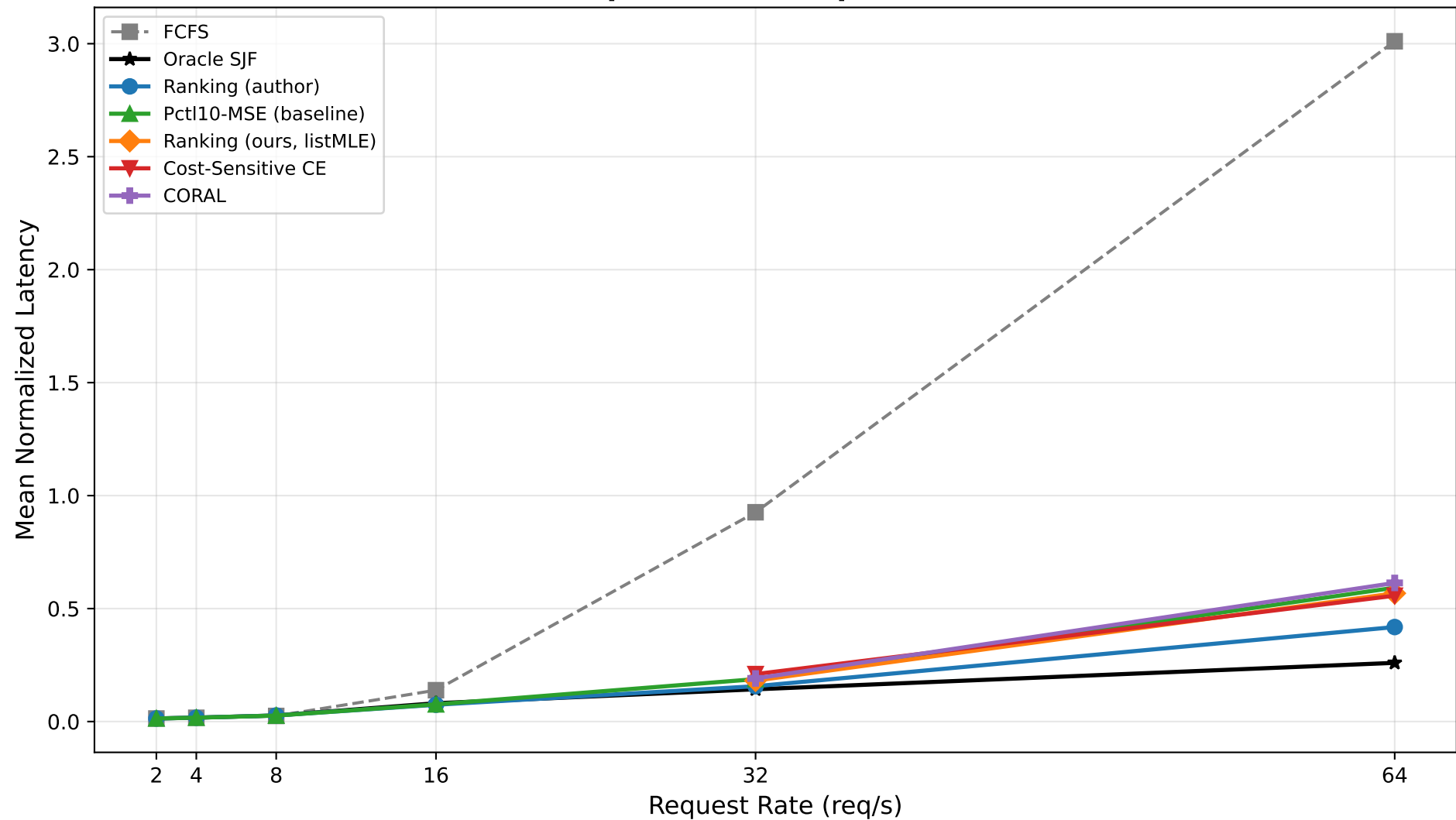
B4 Loss Experiment Comparison — LMSYS
