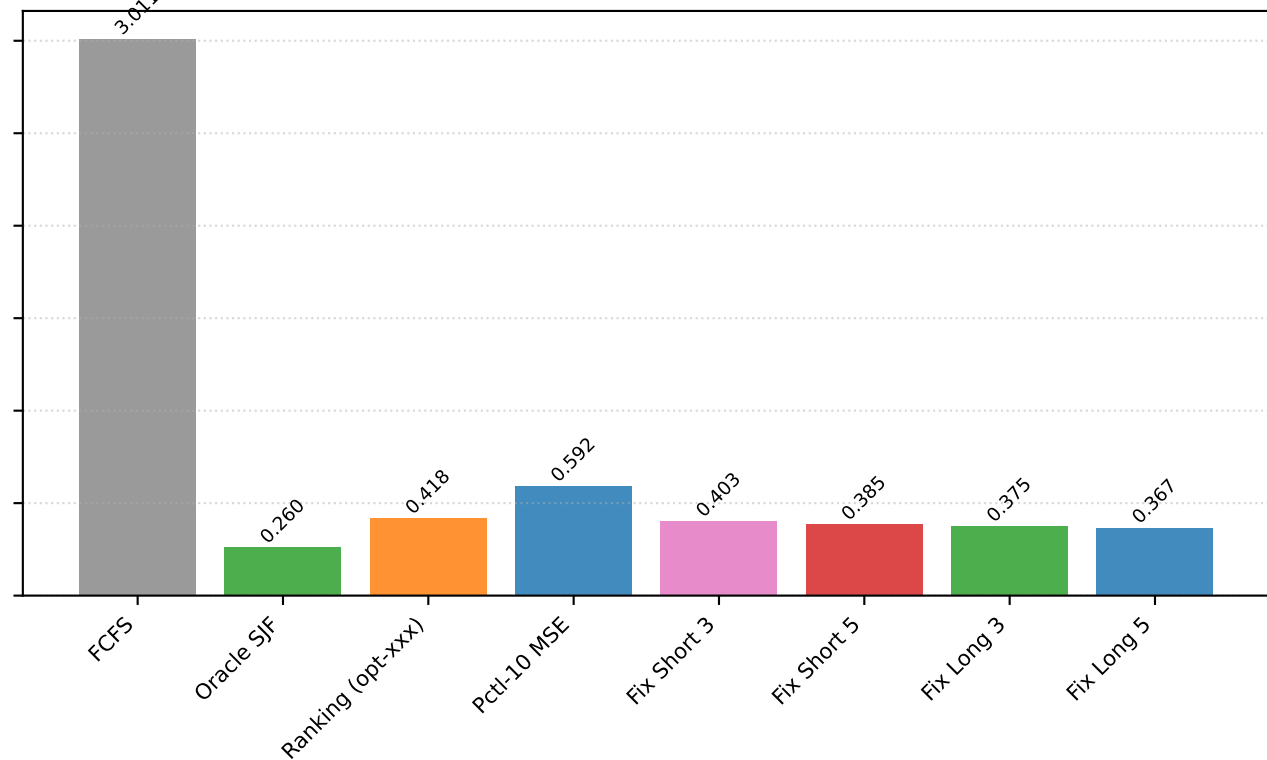
ShareGPT — rate=64
