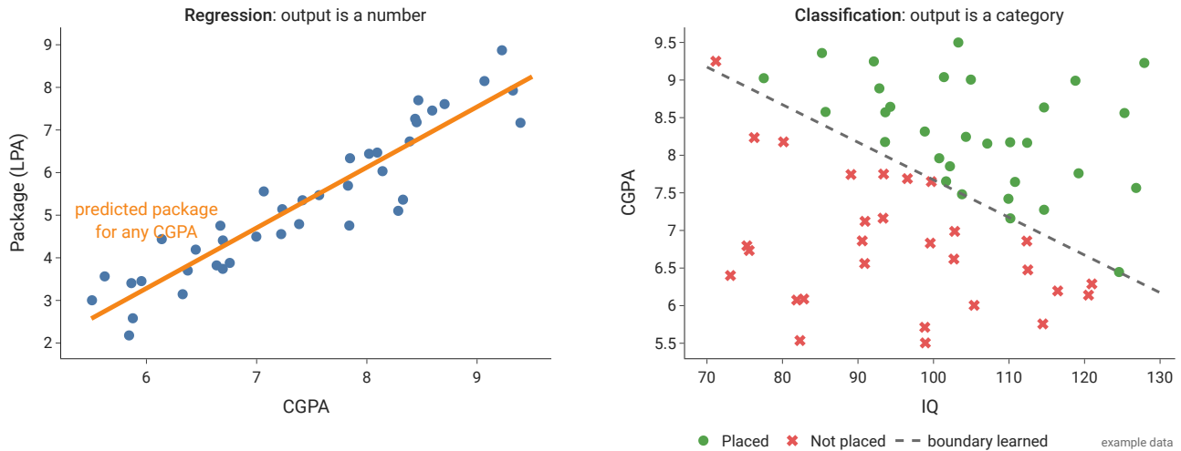
Figure 3: Regression vs classification
