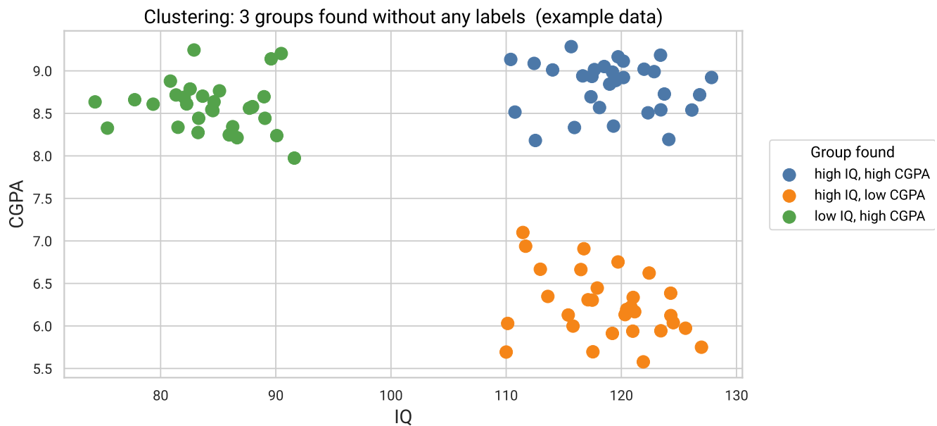
Figure 4: Clustering: groups found without labels
