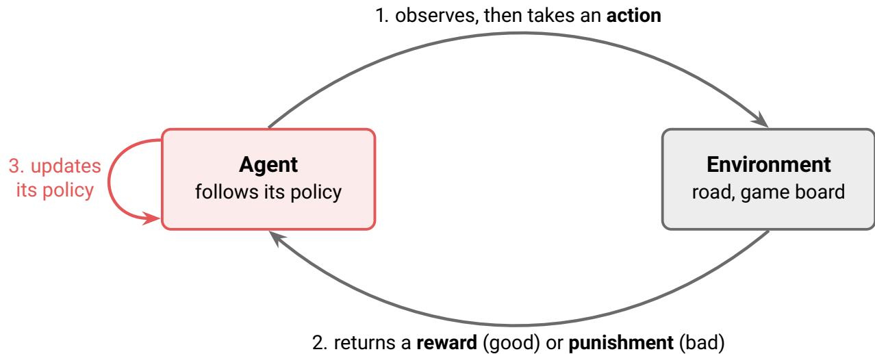
Figure 10: The reinforcement learning loop
