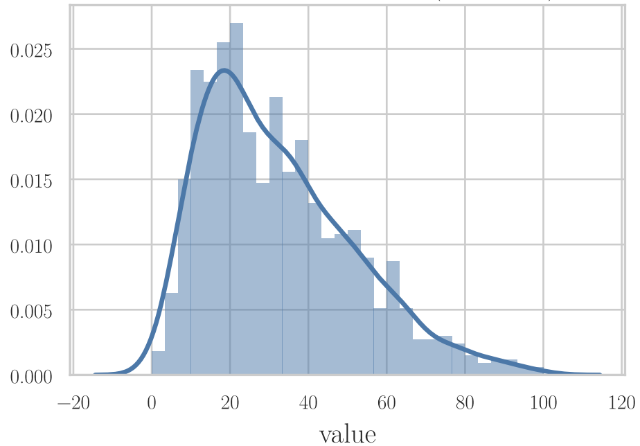
placement_exam_marks (skew 0.84)
