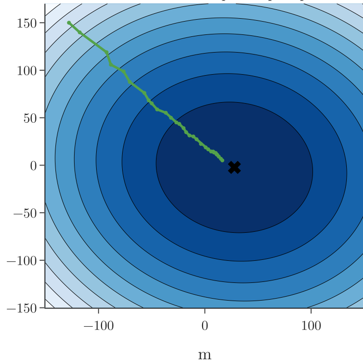
Mini-batch of 10: 10 updates per epoch
