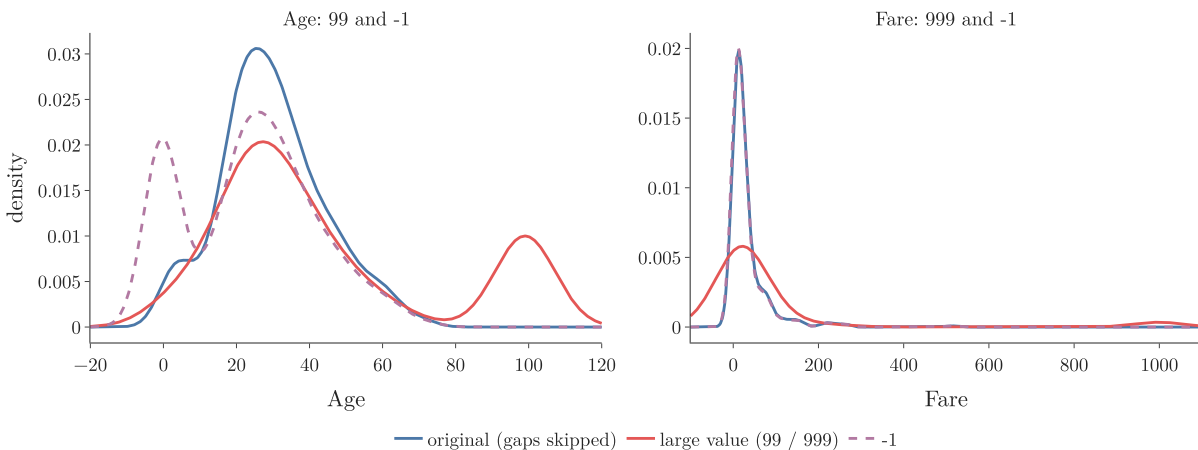
Figure 5: Density of Age and Fare after arbitrary value imputation: a new hump appears at 99 or at -1
