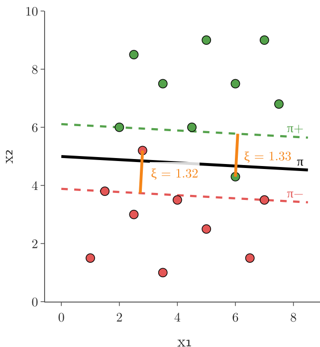
Figure 2: The slack \xi of the two points that break their constraints (orange); all other points have \xi = 0
