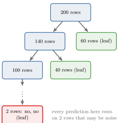
Figure 1: (a) A fully grown tree ends in tiny leaves; (b) a tree of depth 1 stops after one question
