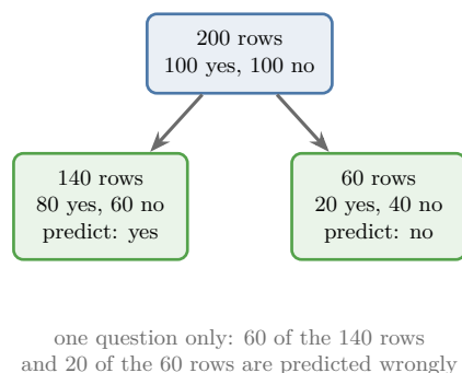
(b) max_depth = 1: underfitting
