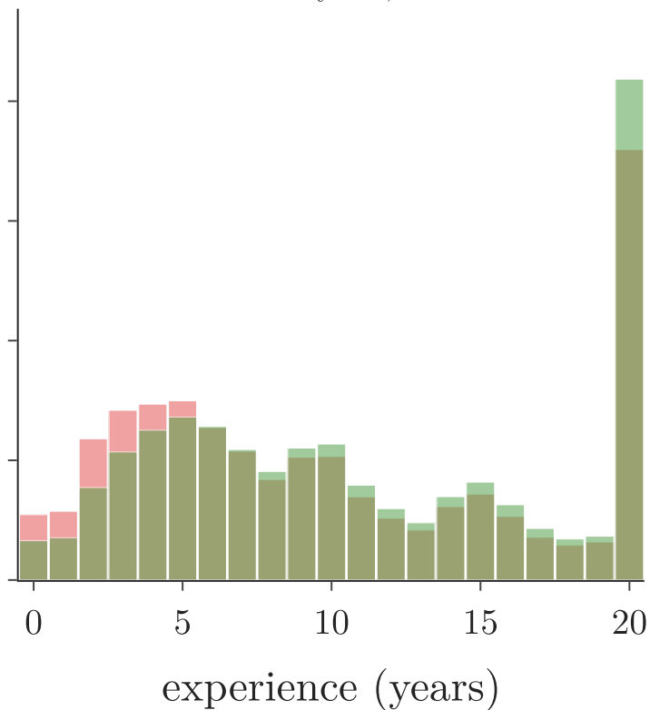
MAR: 80% hidden if no relevant experience mean 9.9 to 11.0 years, 22% removed
