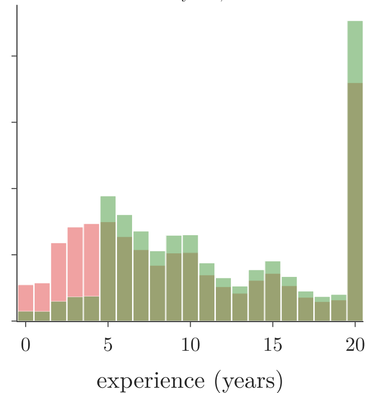
MNAR: 80% hidden if under 5 years mean 9.9 to 11.9 years, 21% removed
