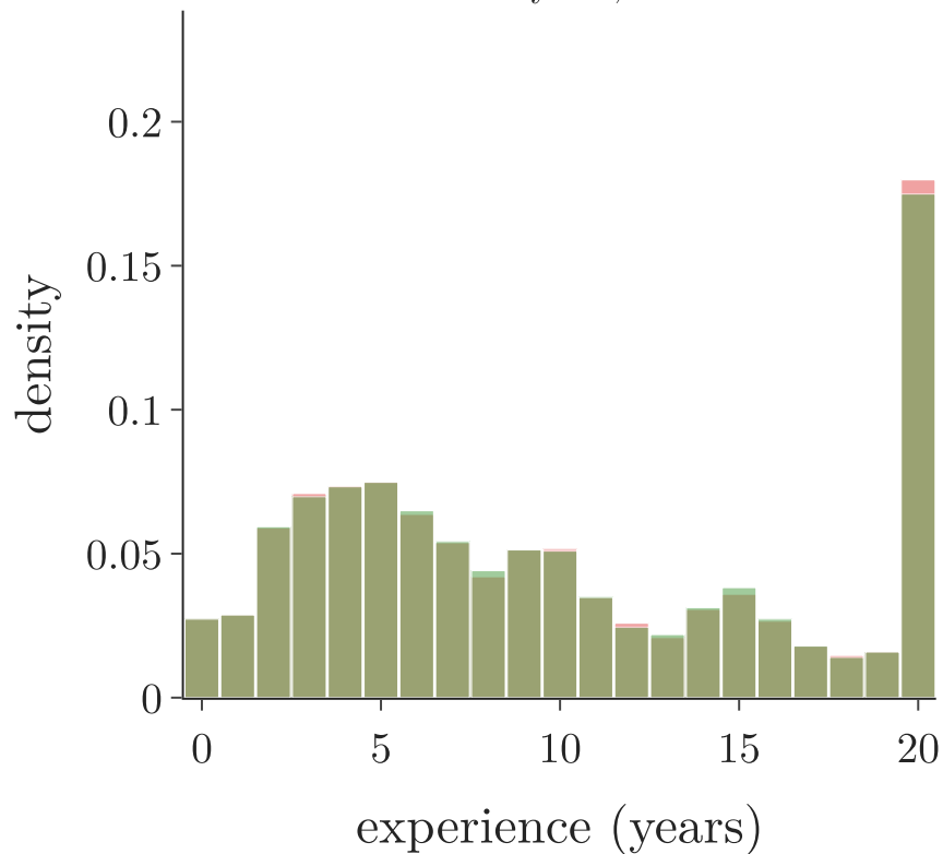
MCAR: 25% hidden at random mean 9.9 to 9.9 years, 25% removed
