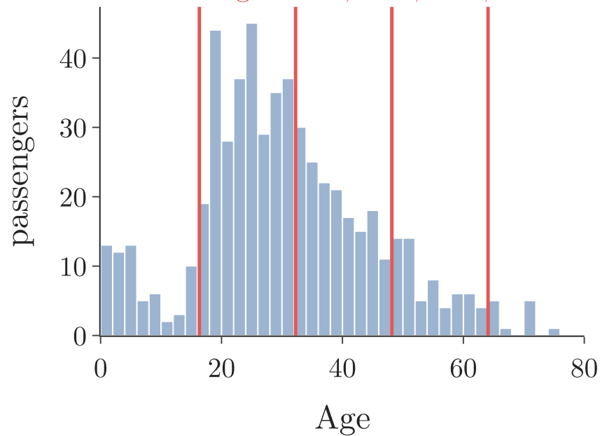
Equal width (uniform)
