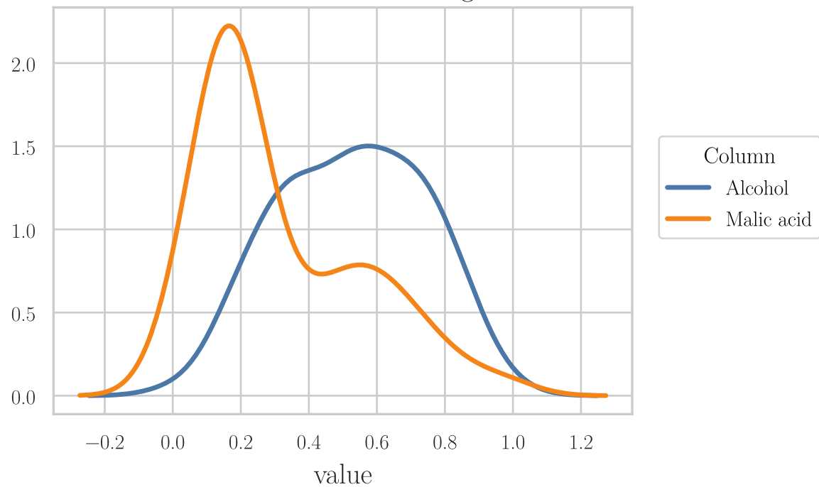
After min-max scaling
