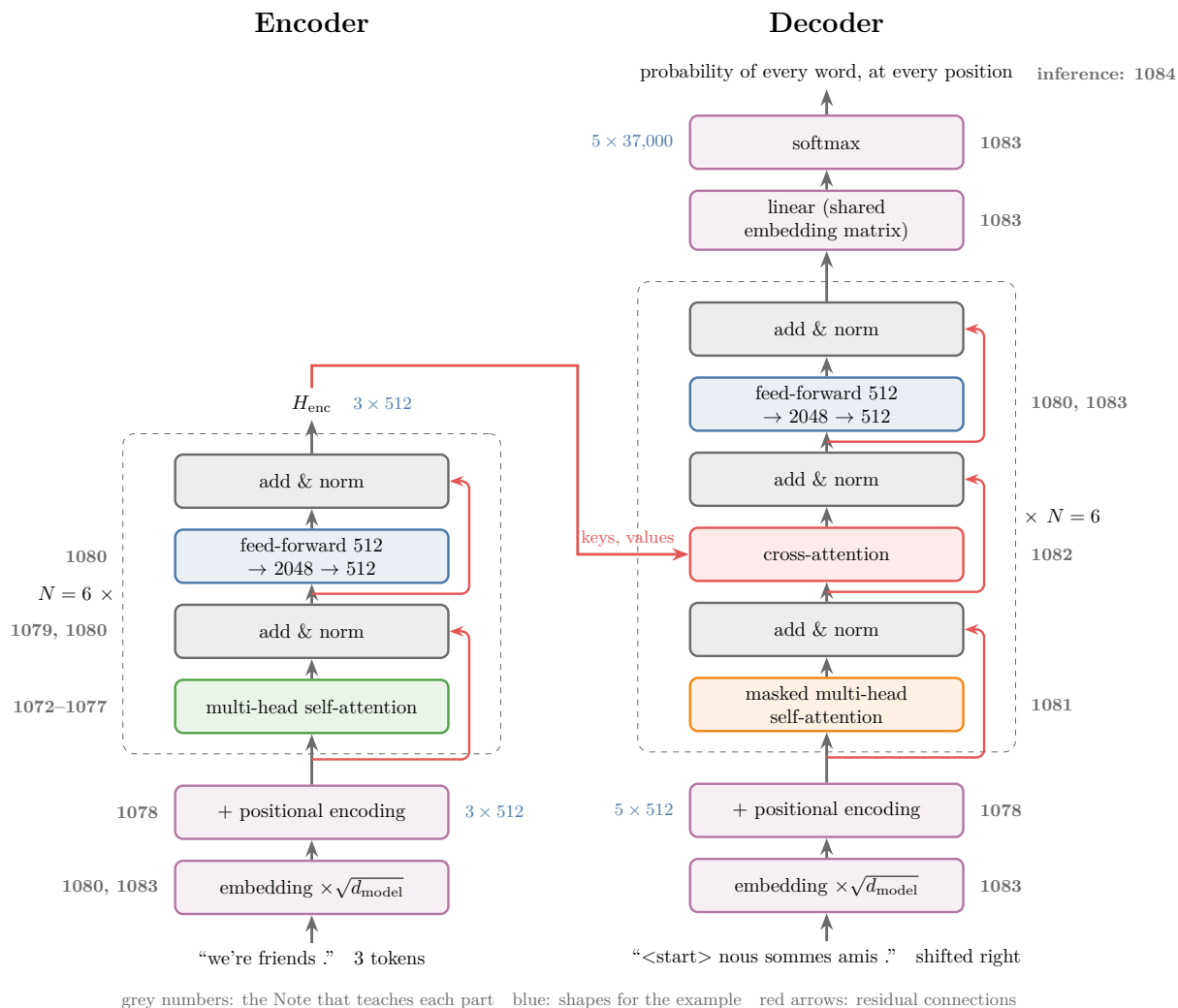
Figure 1: The transformer, base model. Grey numbers: the Note that teaches each part. Blue: the shapes for "we're friends ." \rightarrow "nous sommes amis ."
