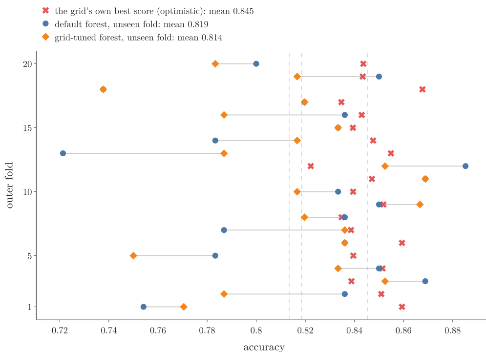
Figure 6: Nested cross-validation on the heart data, 20 outer folds: the default forest (blue) and the grid-tuned forest (orange) scored on data the search never saw, joined by a grey line per fold, and the grid’s own best inner score (red cross); dashed lines mark the means
