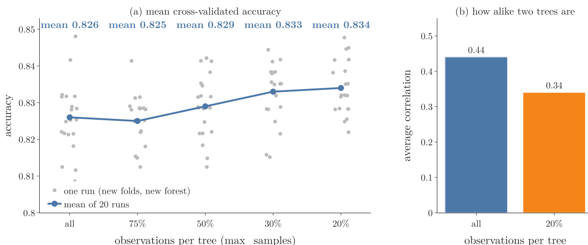
Figure 5: (a) Mean 10-fold cross-validated accuracy against the observations per tree ( max_samples ), 500 trees; each grey dot is one of 20 runs with new folds and a new forest. (b) Average correlation between two trees' predicted probabilities on the 61 test patients
