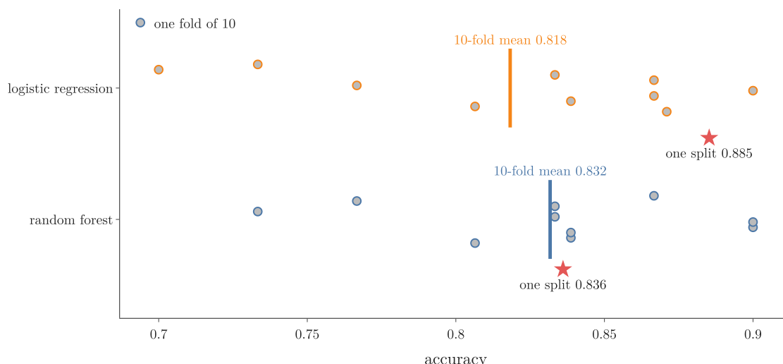
Figure 4: One test split (red star) against the 10 folds of 10-fold cross-validation (dots) for the random forest and logistic regression on the heart data; the bar marks the mean of the 10 folds
