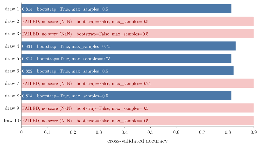
Figure 7: The 10 combinations a naive RandomizedSearchCV drew from one big grid on the heart data: blue bars are the cross-validated accuracies of those that ran; pink rows failed with no score
