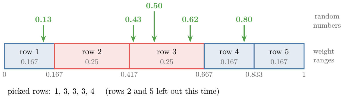
Figure 5: Upsampling: each observation owns a stretch of the line from 0 to 1 as long as its weight; five random numbers pick observations 1, 3, 3, 3 and 4
