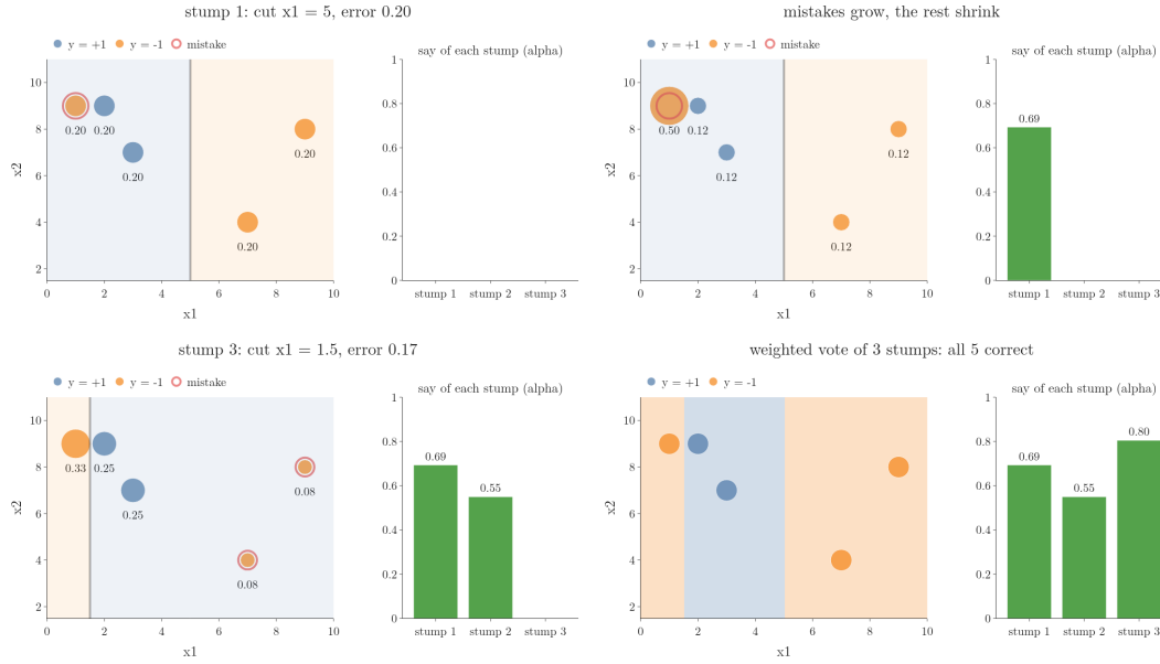
Figure 6: Three AdaBoost stages on the toy data. Dot size and label: the observation's weight. Line and shading: the stump's cut and the class on each side; red rings: its mistakes. Right: each stump's alpha. Last frame: the sign of the weighted vote.
