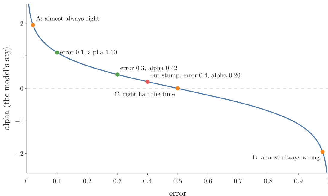
Figure 3: Alpha against the error: model A (error near 0) gets a large positive say, model C (error 0.5) none, model B (error near 1) a large negative say; red: the stump of this Note; green: two stumps with fewer mistakes
