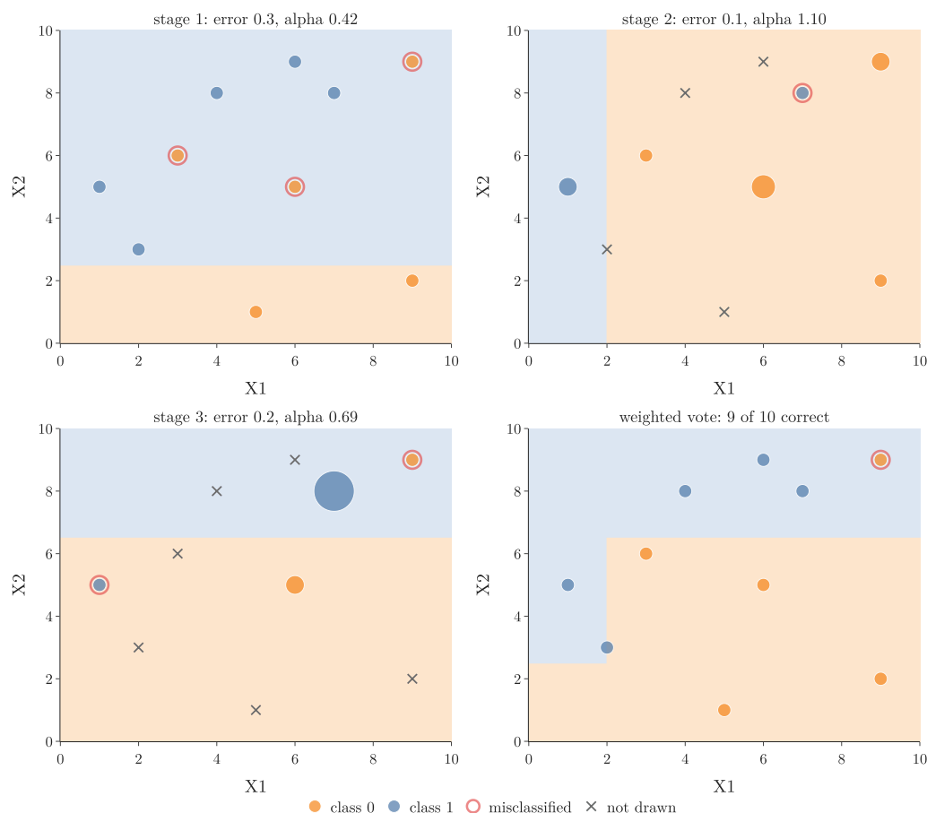
Figure 1: Three stages of AdaBoost on the 10-observation toy data, and their weighted vote. Marker size shows how many copies of an observation are in that stage's dataset; crosses are observations not drawn
